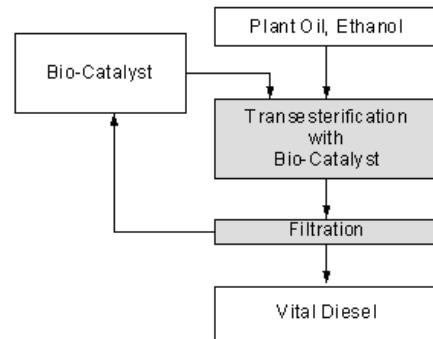
The Vital Diesel process with a fuel yield of >99.9% - new, simple, clean process
