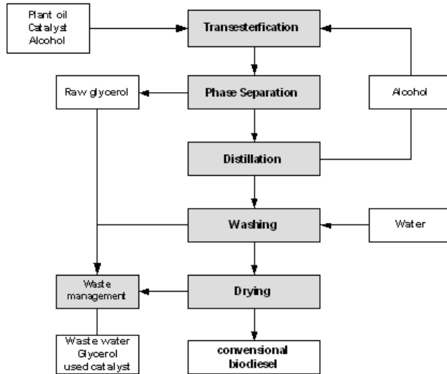
The conventional biodiesel process with a fuel yield of 89% - old, suboptimal process
